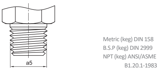
Form C (DIN 3852 Part 1&2) with sealing in tapered thread
